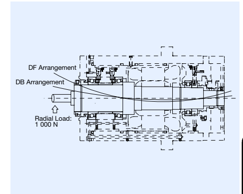
Fig. 3.4 Spindle Displacement Curve
